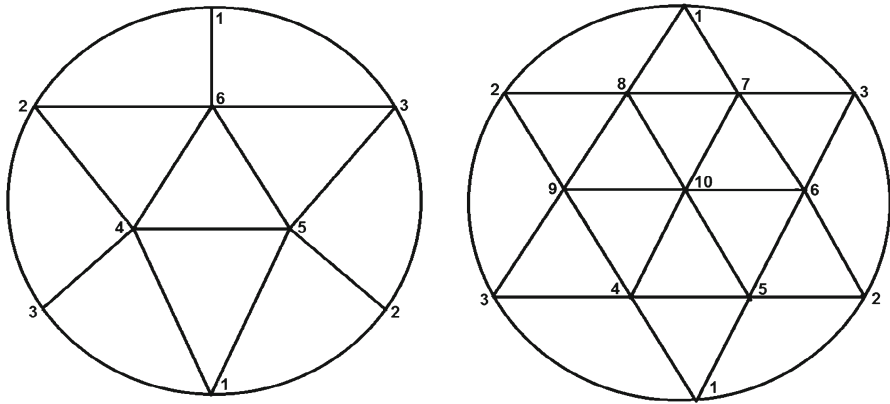
Fig. 2 The standard 6 point triangulation of the real projective plane, and a modified 10 point triangulation
