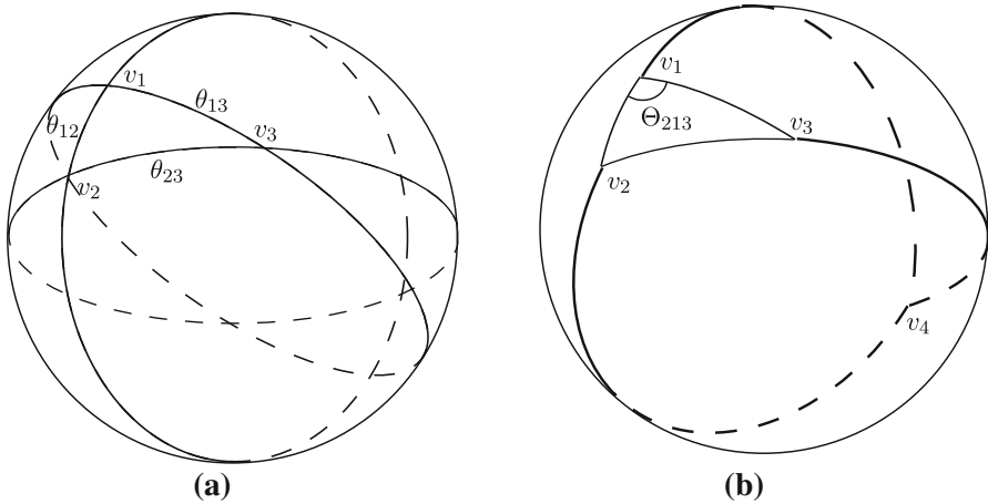
Fig. 2 a Spherical triangle constructed with three great circles. b Partition of the sphere into four spherical triangles.
