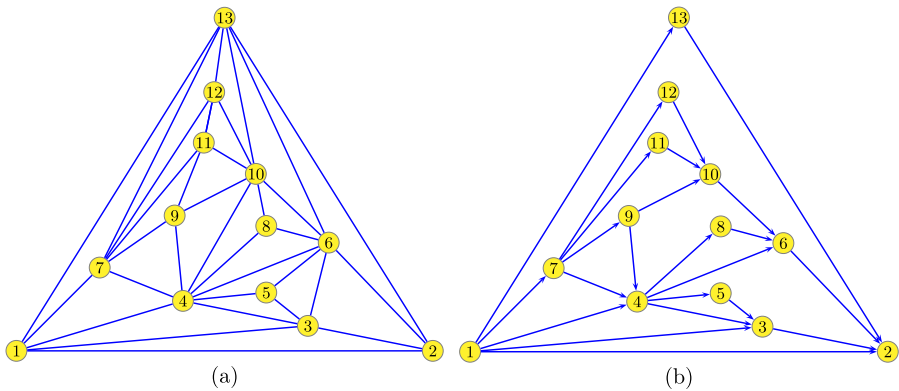
Fig. 2 Illustration for the proof of Theorem 18: (a) Canonical ordering of G , (b) Frame \mathcal{F} of G
