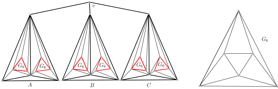
Fig. 1 Illustration for the proof of Theorem 16
