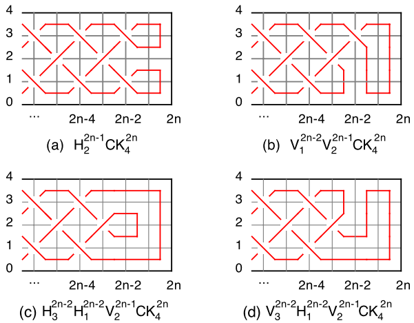
Fig. 8 Celtic diagrams for bracket polynomial relations
