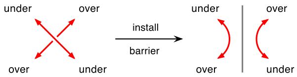
Fig. 2 Installing a barrier in an alternating link diagram
