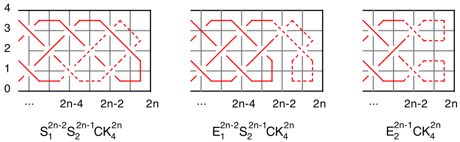
Fig. 7 Iterative operations on CK_4^{2n}
