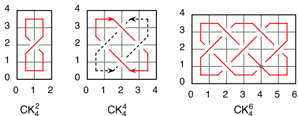
Fig. 5 Some small barrier-free 4 \times c Celtic knots
