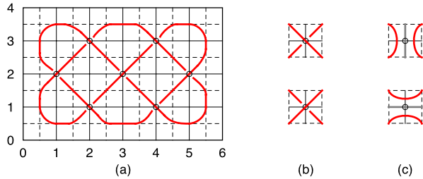
Fig. 1 Drawing a Celtic knot
