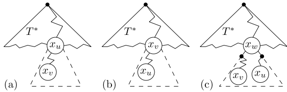
Fig. 1 All elements x_z, z \in \bar{S} , are stored in a subtree rooted at x_w . (a) If w = u , then I_{uv} = 0 ; (b) if w = v , then I_{uv} = 1 ; and (c) if w \in S_{uv} , we have I_{uv} = 0
