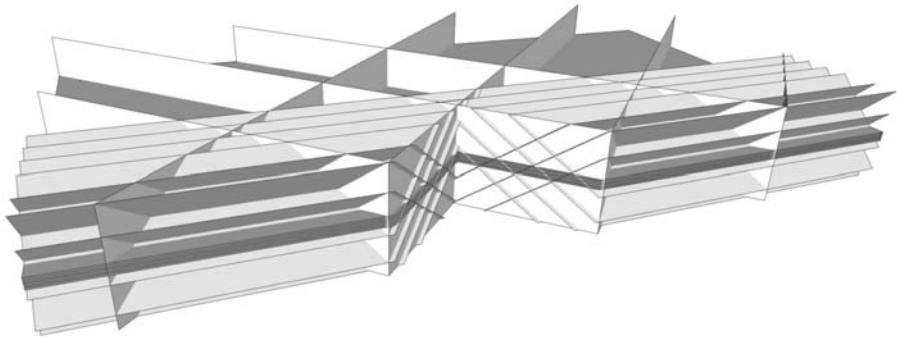
Fig. 7 The affine arrangement \mathcal{A}_4 consists of three families of planes: The first family \mathcal{A}'_3 \times \mathbb{R} forms a coarse vertical grid; the second family (derived from \mathcal{H}_3 \times \mathbb{R} by tilting) forms a finer grid running from left to right; the last family \mathcal{H}_4 contains the parallel horizontal planes
