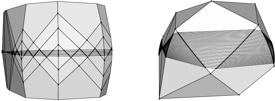
Fig. 8 Two different projections of a dual 4-zonotope with cubic 2D-shadow. On the left the projection to the first two and last coordinate (clipped in vertical direction) and on the right the projection to the first three coordinates
