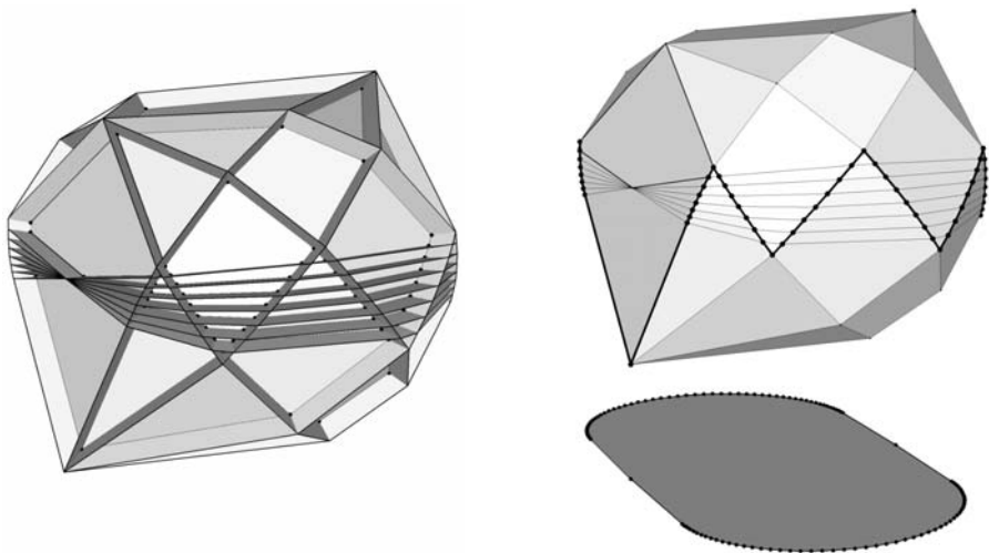
Fig. 5 A dual 3-zonotope with quadratic 2D-shadow, on the left with the corresponding linear arrangement and on the right with its 2D-shadow
