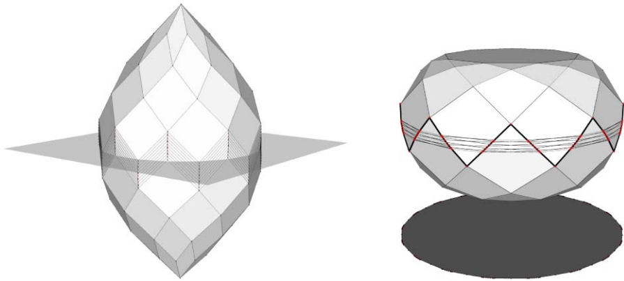
Fig. 1 Eppstein's Ukrainian easter egg and its dual. The 2D-cut, resp. shadow boundary, of size \Omega(n^2) are marked
