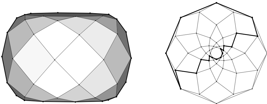
Fig. 4 Shadow boundary of a centrally symmetric 3-polytope, on the right displayed as its Schlegel diagram
