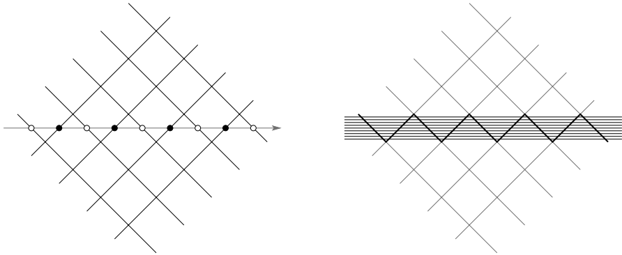
Fig. 6 Constructing the arrangement \mathcal{A}'_3 from \mathcal{A}_2 (left) and \mathcal{A}_3 from \mathcal{A}'_3 (right)
