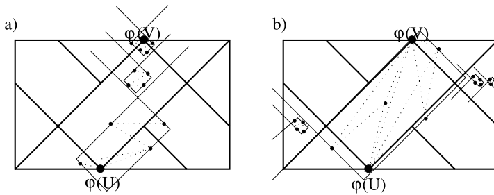
Fig. 4 Two examples of embeddings. In (a), the components move within the X-dimension and in (b) the components move within the Y
