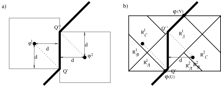
Fig. 3 The bold line in (a) gives the set of points Q whose distances to C' is equal to its distance to C'' . (b) Demonstrates how this region lies within completely in the region S
