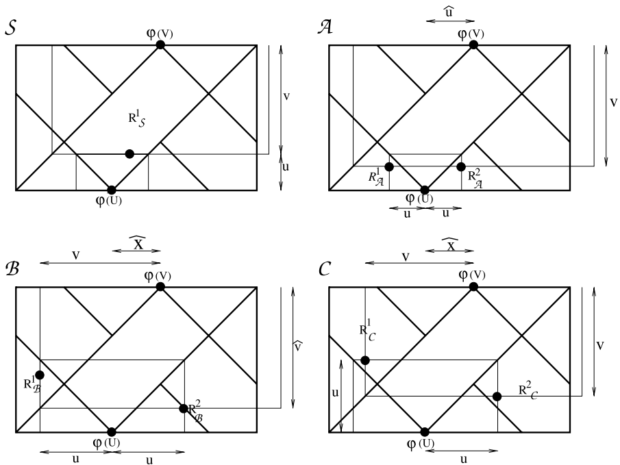
Fig. 2 For each classification of points P , it is shown how the square around U and that around V intersect at two regions
