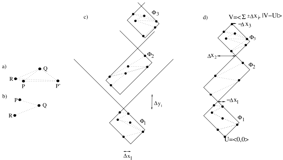
Fig. 5 (a) and (b) Fixing points within a component. (c) The relative placements of the components \Phi_1 , \Phi_2 , and \Phi_3 . The edges with the components are shown. (d) The metric space corresponding to the Subset Sum problem
