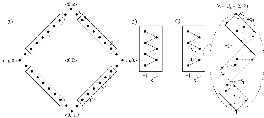
Fig. 6 (a) In two of the dimensions the points of the Möbius metric space form a square. (b) Along each edge of the square the points zig-zag between X -coordinates 1 and -1 . The edges between the nodes are those used in Lemma 3 for fixing the last dimension. We first prove that the nodes within the long rectangles in both (a) and (b) are fixed to form connected components. Then we show that all the points form a single connected cycle. (c) Shows how the metric space from Theorem 2.3 is later inserted into this metric space in order to prove Theorem 2.1
