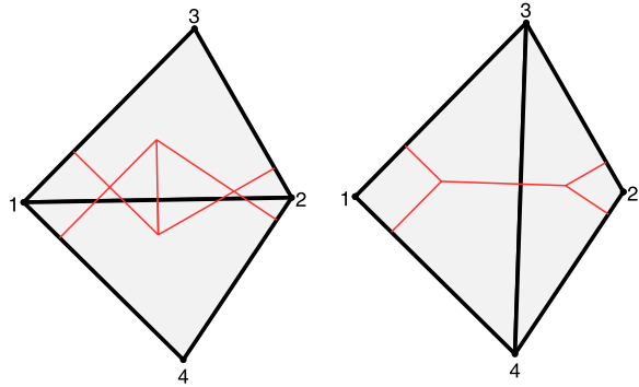
Fig. 1 Hinges \mathcal{T} and \mathcal{T}' differing by a bistellar flip. The dual edges are also shown
