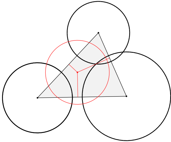
Fig. 2 A weighted triangle with circles corresponding to the weights at the vertices. Central orthogonal circle and dual edges are also shown
