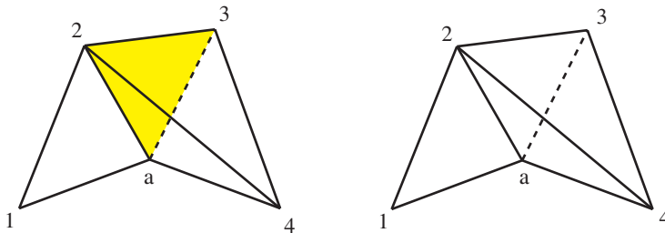
Fig. 4. Removing pseudoflip.
