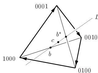
Fig. 4. The winding number with respect to L .
