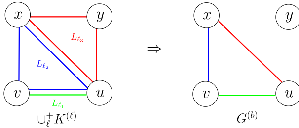
Fig. 1 Weighted intersection graph as a multigraph composed by 3 overlapping cliques K^{(l_1)} \cup^+ K^{(l_1)} \cup^+ K^{(l_3)} (left) and graph G^{(b)} constructed by the Weak Bipartization Algorithm, consisting of a closed vertex-label sequence \sigma^{(\text{odd})} = x, l_2, v, l_1, u, l_3, x (right)
