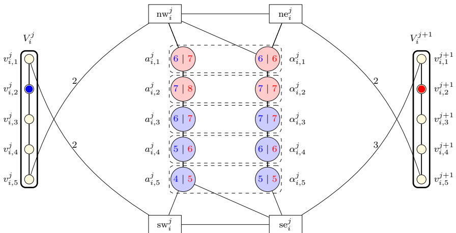
Fig. 3 The propagation gadget P_i^{j,j+1} . The critical pairs \{\alpha_{i,\gamma}^j, \alpha_{i,\gamma}^{j+1}\} are surrounded by thin dashed lines. The blue (resp. red) integer on a vertex of A_i^j is its distance to the blue (resp. red) vertex in V_i^j (resp. V_i^{j+1} ). Note that the blue vertex distinguishes the critical pairs below it, while the red vertex distinguishes critical pairs at its level or above (Color figure online)
