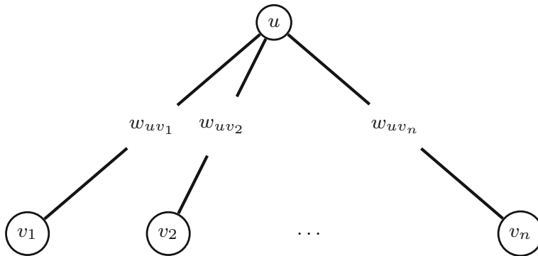
Fig. 1 An instance of PG on a star
