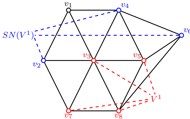
Fig. 4 Significant neighbours SN(V^1) = \{v_2, v_4, v_6\} of V^1 = \{v_3, v_5, v_7, v_8\} in the graph of solid black lines
