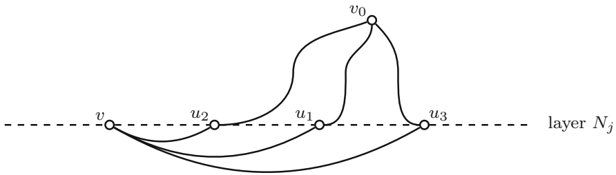
Fig. 7 Relations between N_j and N_j
