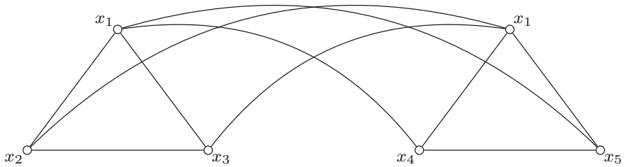
Fig. 2 Illustration of the reduction
