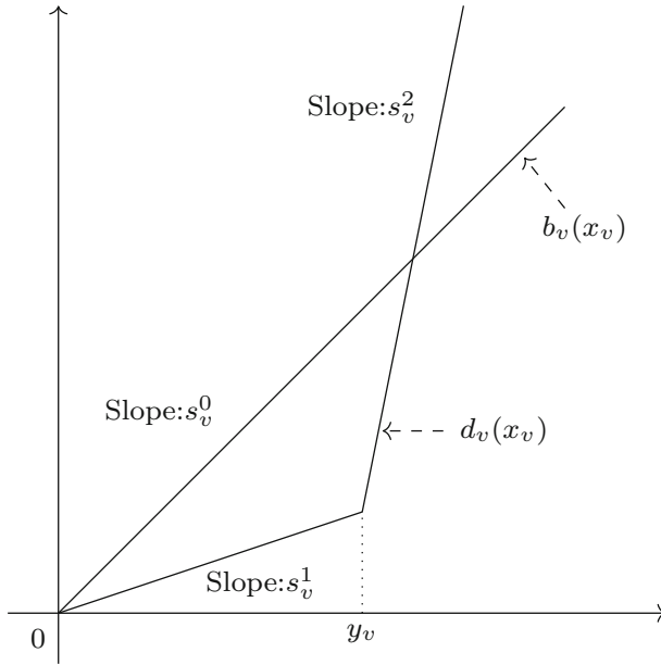
Fig. 9 An illustration of function b_v and d_v
