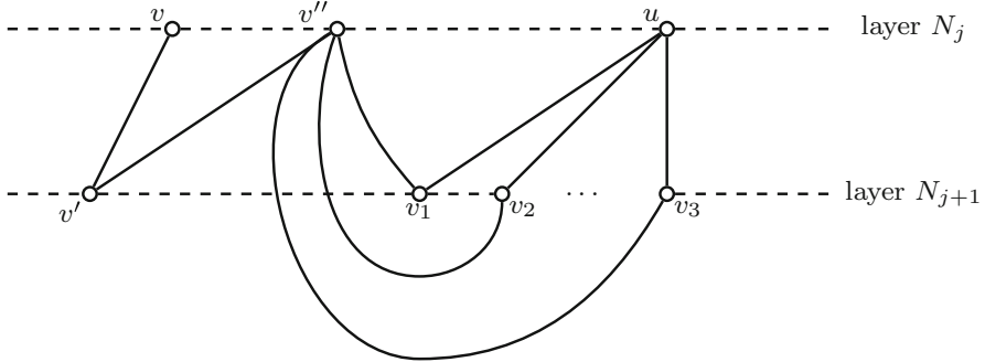
Fig. 6 Relations between N_j and N_{j+1}
