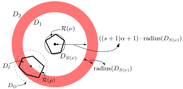
Fig. 1 Illustrating the proof of Lemma 16 (in 2D)
