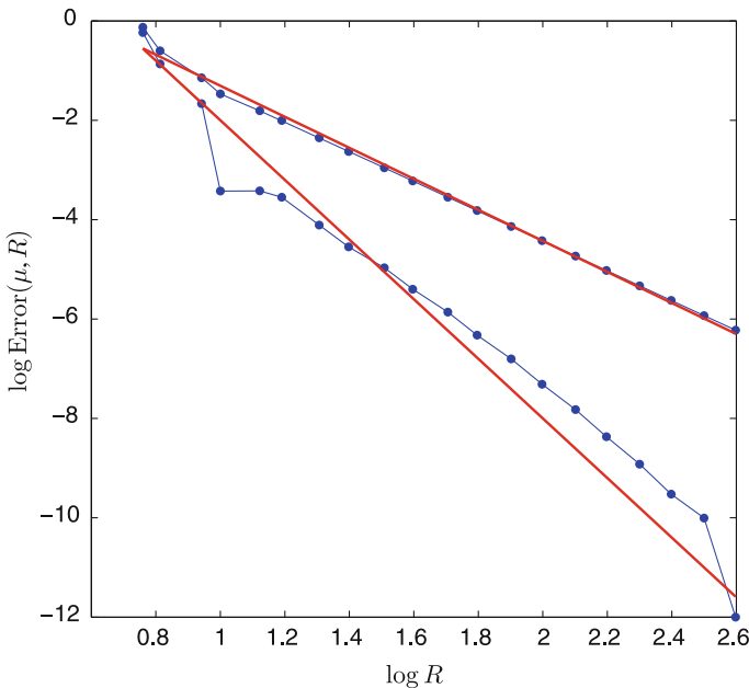
Fig. 2 Absolute error in log scale for \mu = 250 R^{-3/2} , A_{\mu,1,R,L} (slope -3.1 ) and A_{\mu,2,R,L} (slope -6 ), filter of infinite order
