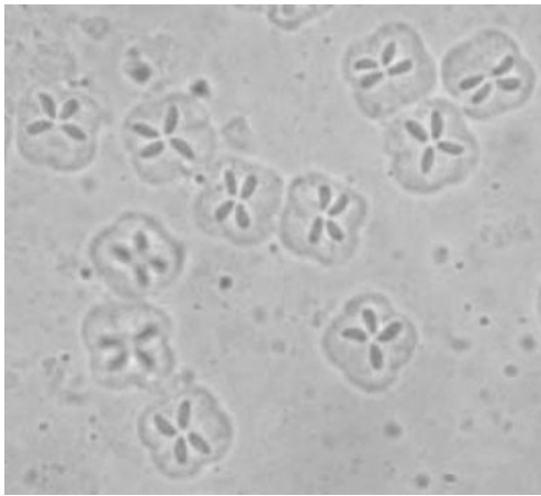
Photomicrograph of fresh spores of Kudoa pagrusi
