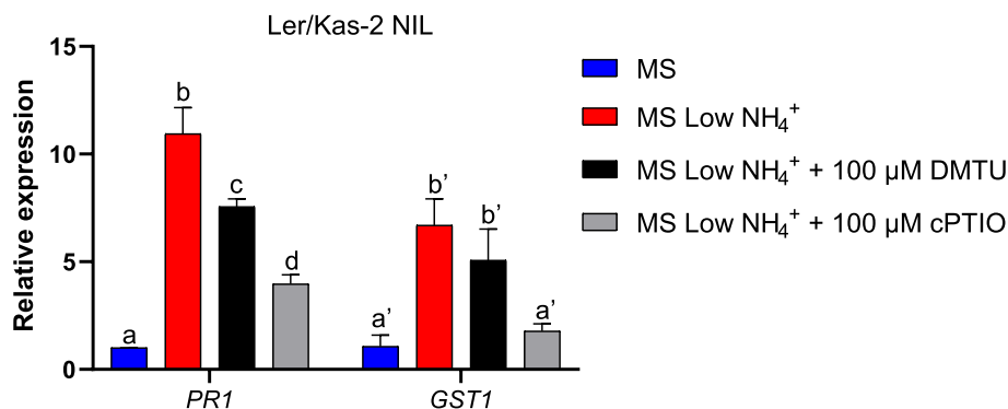
Fig. 9 Quantitative gene expression analyses of PR1 and GST1 in Ler/Kas-2 NIL plants grown in vitro on MS or low ammonium MS at 14–16 °C and treated with 100 \mu\text{M} DMTU (1,3-dimethyl-2-thiourea) or 100 \mu\text{M} cPTIO [2-(4-carboxyphenyl)-4,4,5,5-tetramethylimidazo-
