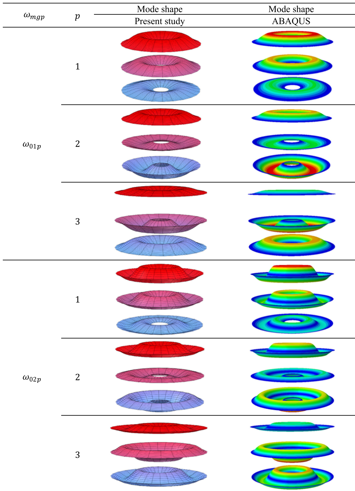
Fig. 4 Some of the mode shapes of the system
