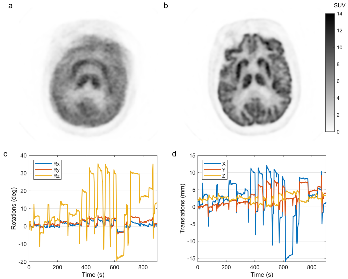
Fig. 1 ^{18}\text{F} -Fluorodeoxyglucose, axial PET image at the level of the basal ganglia with significant blurring due to movement (a). Corresponding axial PET image, corrected for motion (b), all other recon-
