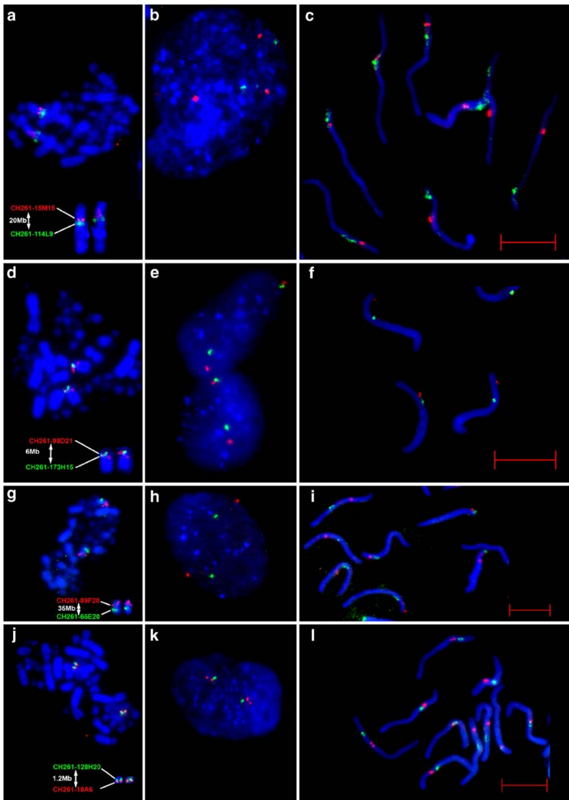
Fig. 3 Mapping of chicken BACs in chicken cells. Using two-color FISH, we localized chromosomes in mitotic metaphase ( a , d , g , h ), interphase ( b , e , h , k ), and sperm ( c , f , i , l ). Examples are shown for BACs CH261-15M15 (114 Mb, green ) and CH261-114L9 (134 Mb, red ) from GGA 1, ( a , b , c ), BACs CH261-98D21 (10 Mb, red ) and
