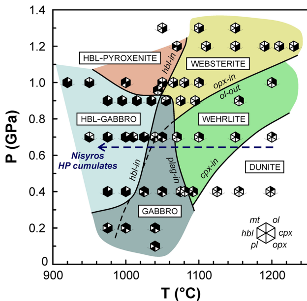
Fig. 10 Phase diagram for hydrous ( \geq 3 wt% H_2O in starting material at fO_2 \geq NNO ) primitive arc magmas, modified after Melekhova et al. (2015) to include data from additional experimental studies (Müntener et al. 2001; Pichavant and Macdonald 2007; Blatter et al. 2013; Nandedkar et al. 2014; Andújar et al. 2015). The Nisyros Type 2 and 3 cumulates evolve from (hornblende-)wehrlites to hornblende-gabbros and plagioclase-hornblendites, consistent with crystallisation at 0.5–0.8 GPa (blue arrow). See text for further discussion
