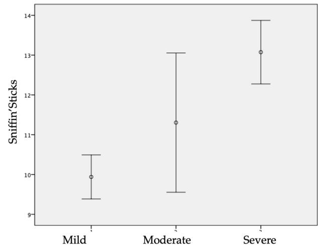
Fig. 3 Mean and standard deviation of Sniffin'Stick test values according to the severity group
