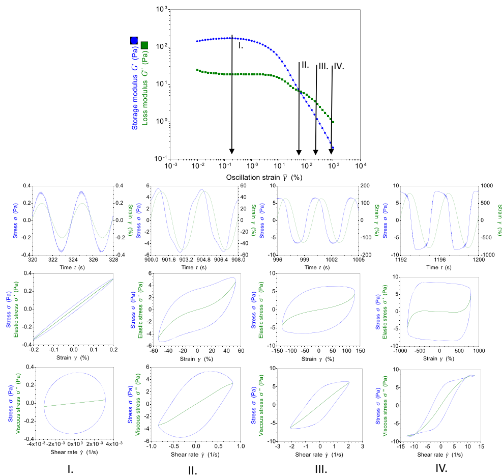
Fig. 1 Strain sweep of YD-K suspension with dynamic modulus G' and G''
