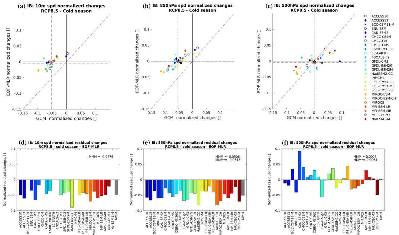
Fig. 11 Same as Fig. 10 but for the Iberia (IB) box
