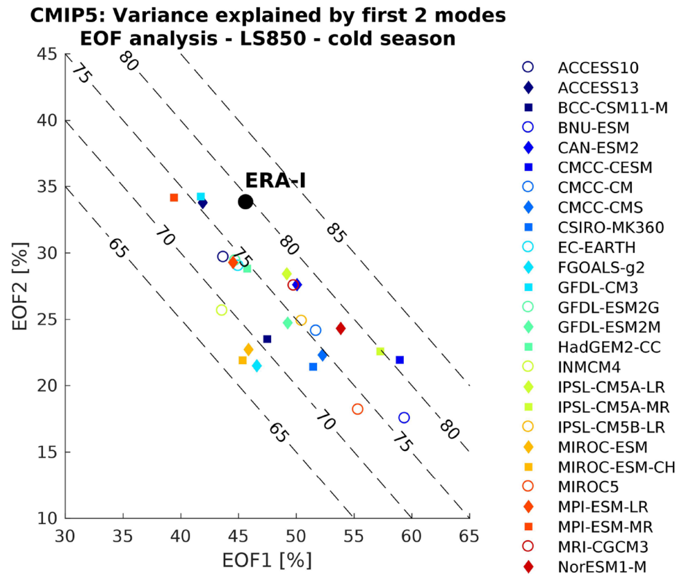
Fig. 4 Summary plot of the EOF analysis applied to the historical CMIP5 ensemble. The x axis presents the variance explained by EOF1 and the y axis for EOF2. Diagonal dashed lines correspond to different amounts of variance accumulated by the two. The black dot represents the values obtained from the ERA-I EOF analysis and individual GCMs are included as different colours and symbols
