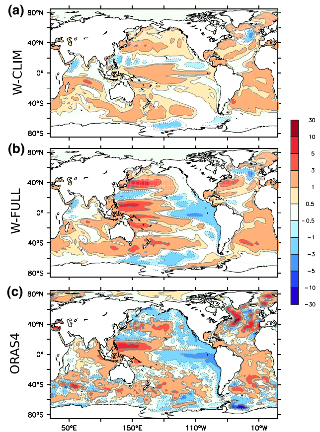
Fig. 6 OHC change over the 1998–2012 period, \Delta\text{OHC} , shown here in 10^9 \text{ J m}^{-2} for the entire ocean column, in a W-CLIM, b W-FULL and c ORAS4
