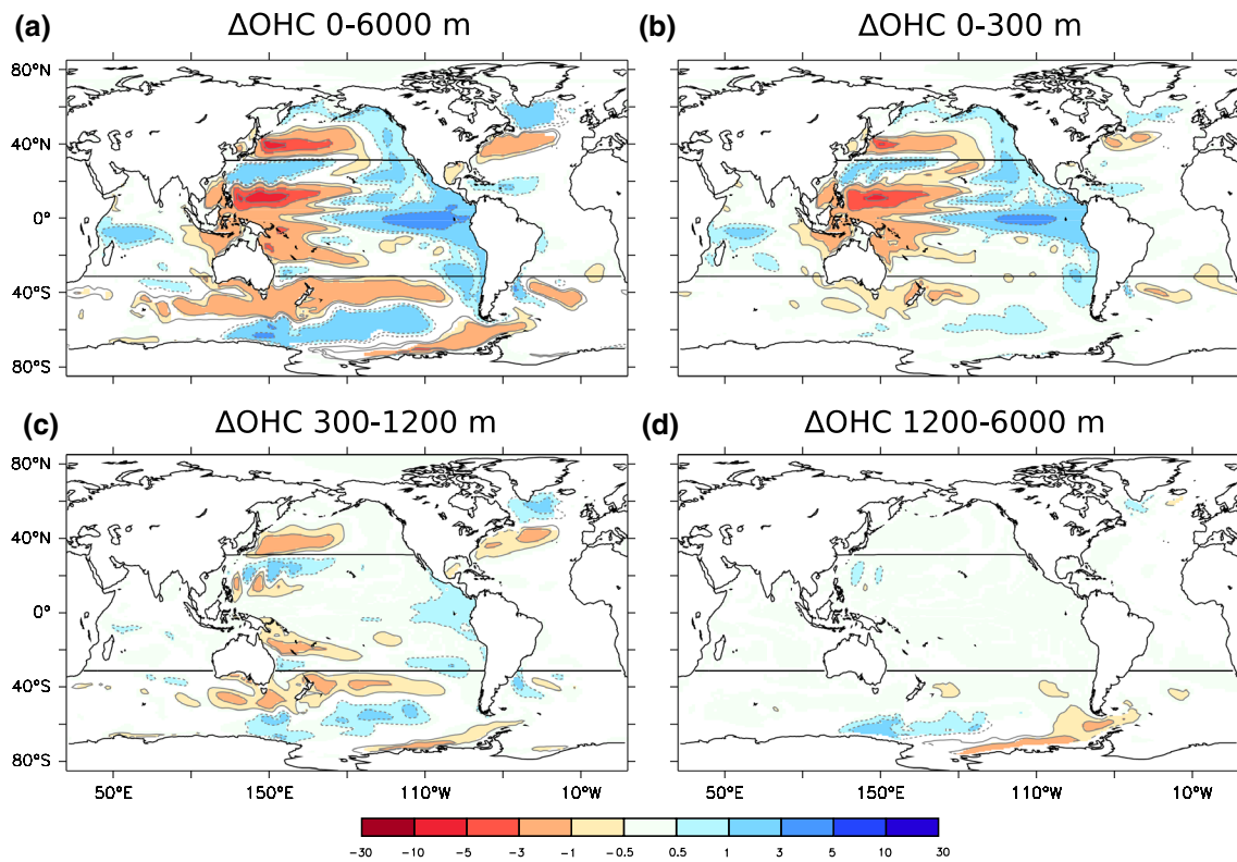
Fig. 7 Vertical distribution of the W-FULL minus W-CLIM OHC change over the 1998–2012 period, \Delta\text{OHC}_{\text{IPO}} , in 10^9 \text{ J m}^{-2} : a entire ocean column, b 0–300 m, c 300–1200 m, and d 1200–6000 m. The
