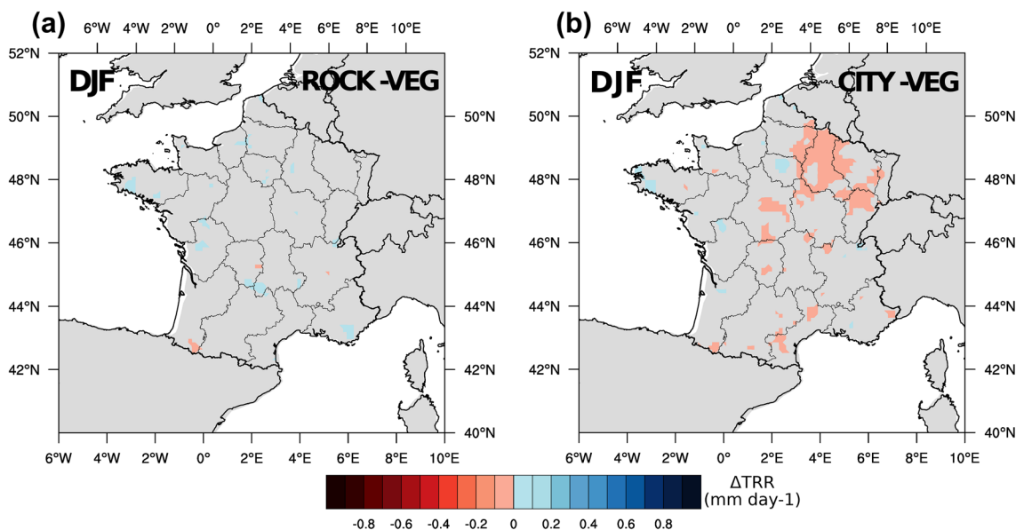
Fig. 6 Differences of precipitation rates (in \text{mm day}^{-1} ) for DJF between ROCK and VEG (a) and between CITY and VEG (b)
