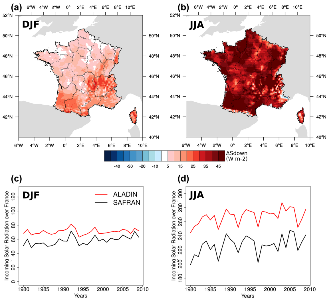
Fig. 3 ALADIN-Climate biases relative to SAFRAN and temporal evolutions (in W m^{-2} ) of the incoming solar radiation for DJF and JJA
