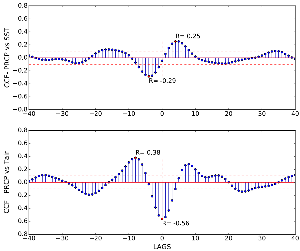
Fig. 9 CCF between SST and P ( upper panel ) and CCF between Tair and P ( lower panel ), using 10–30 day filtered time series. Red horizontal dashed lines indicate 95 % significance level ( N = 4744 ) and
