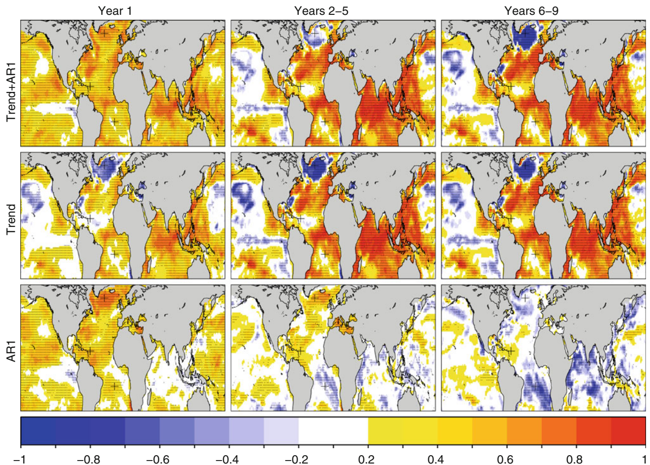
Fig. 3 Correlation measures over different lead time periods for Trend+AR1 and Trend retrospective forecasts with observed anomalies and for AR1 forecasts with the internal variability component of observed anomalies. The forecast time series of grid boxes marked
