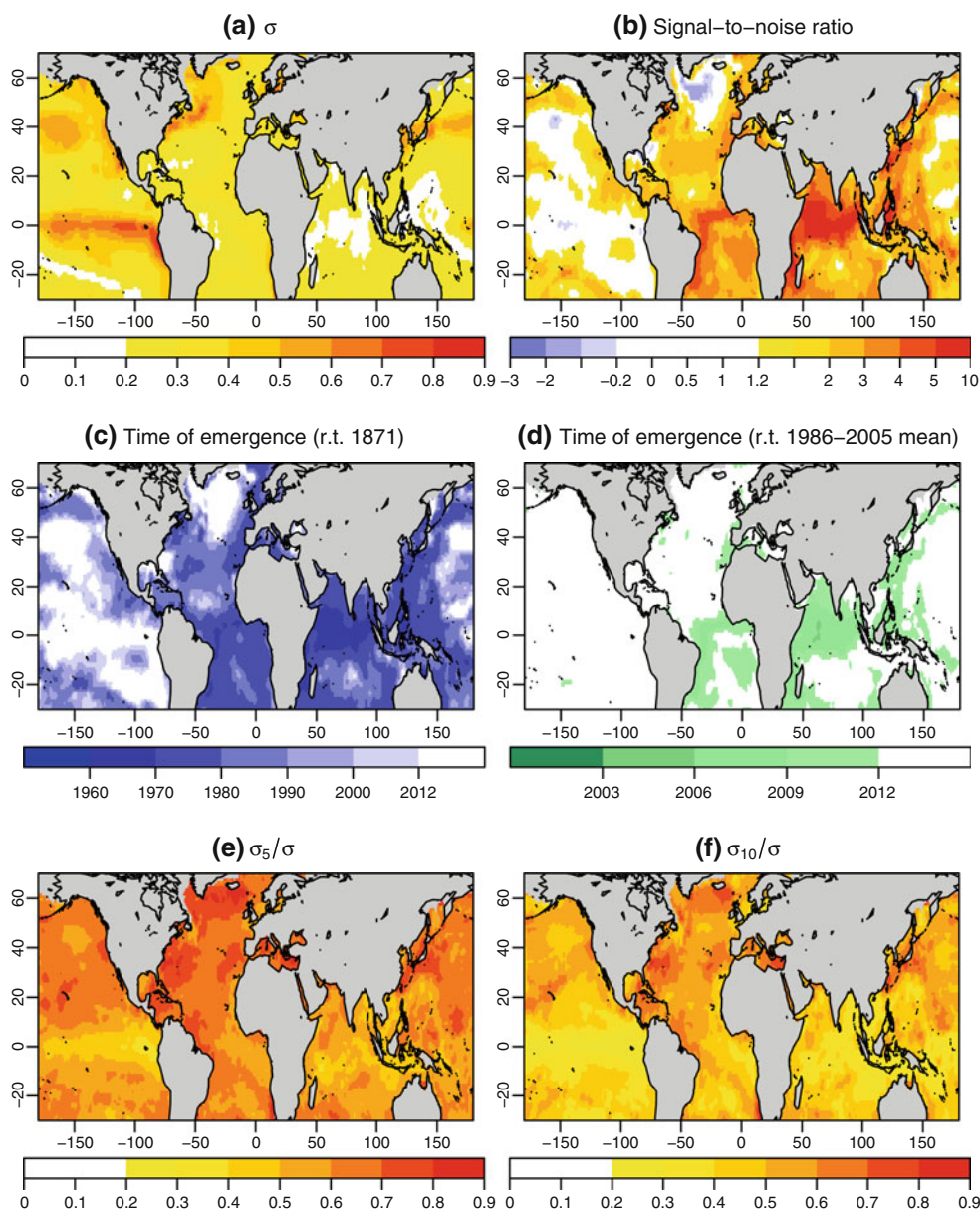
Fig. 2 a Standard deviation of X^v estimated as the residuals of the forced trend regression model (2) (in °C); b Ratio of estimated forced change in SST (signal) to the standard deviation of residuals (noise) of model (2); c and d Time of emergence of climate signal, defined as the year when the signal-to-noise ratio last crossed and exceeded one, relative to (r.t.) two reference baselines (1871 and 1986–2005 mean); e and f Potential predictability as a ratio of the standard deviation of 5 and 10 year means to the standard deviation of interannual variability in SSTs after the forced trend is removed
