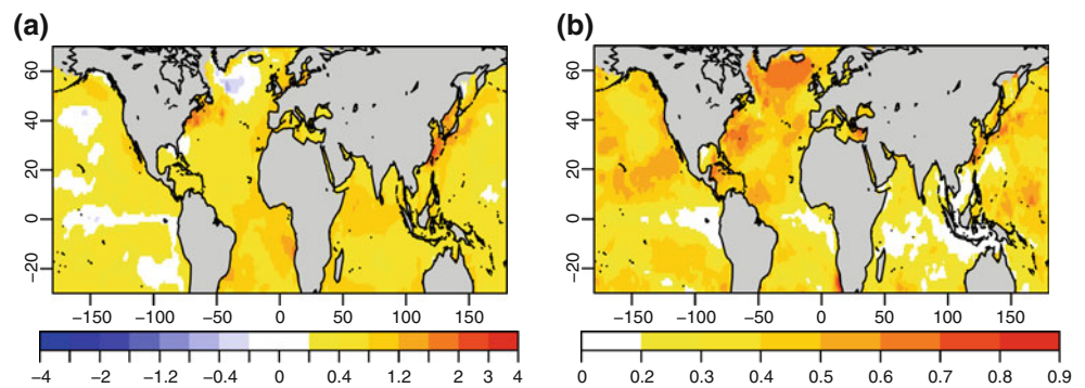
Fig. 1 a Parameter estimate of \alpha_1 in the forced trend regression model (Eq. 2) fitted to data from all available years, representing the dependence of SST on equivalent CO 2 concentration (in °C per 100 ppm); b Estimate of the autoregression coefficient \gamma_1 in the AR1 model (Eq. 4) fitted to data from all available years
