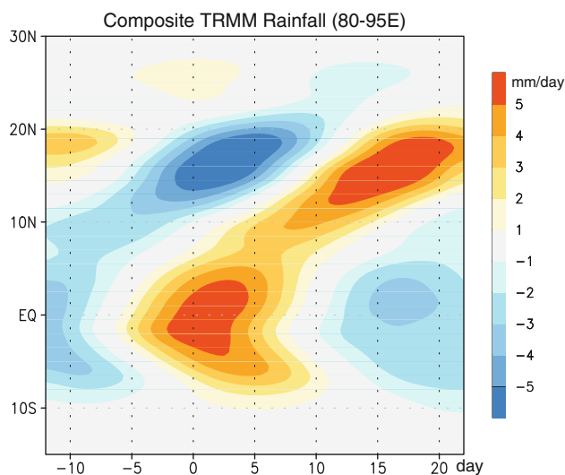
Fig. 2 Time-latitude distribution of composite anomalous rainfall over the BoB sector ( 80^{\circ} – 95^{\circ} E) based on 10 strong BSISV events during 2006–2008 (units: \text{mm day}^{-1} )
