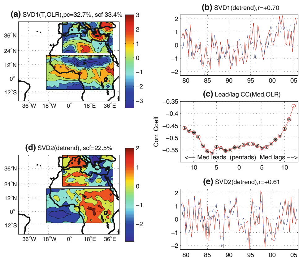
Fig. 1 First and second leading July–September SVD modes performed between skin temperatures in the Mediterranean region and West African OLR values at monthly time step: a, b ( d, e ) describe the first (second) mode in terms of heterogeneous field of covariability and expansion time coefficients while (c) displays lead/lag correlation coefficients between a spatial index averaging surface temperatures in the Mediterranean basin (32–40°N; 6–36°W) and OLR values in the Sahel zone (10–20°N; 15°W–30°E). Values significant at p = 0.05 taking into account autocorrelations in the series are marked by asterisks. Period July–September 1979–2006
