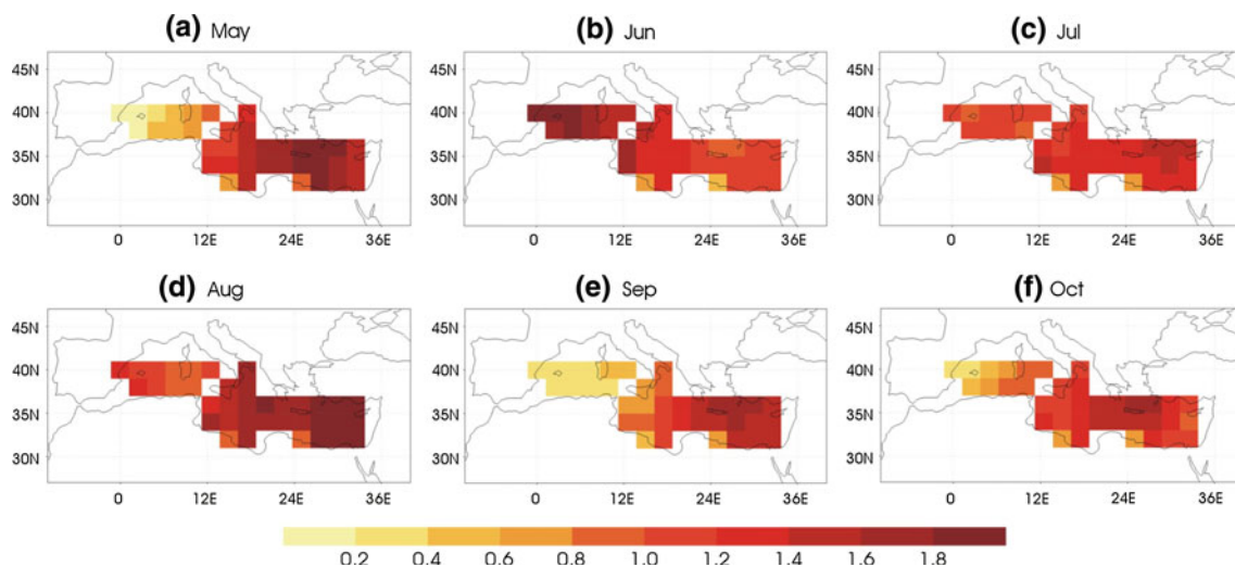
Fig. 5 May–October forcing fields used in the AGCM-sensitivity experiments. SST anomalies are expressed in °C units
