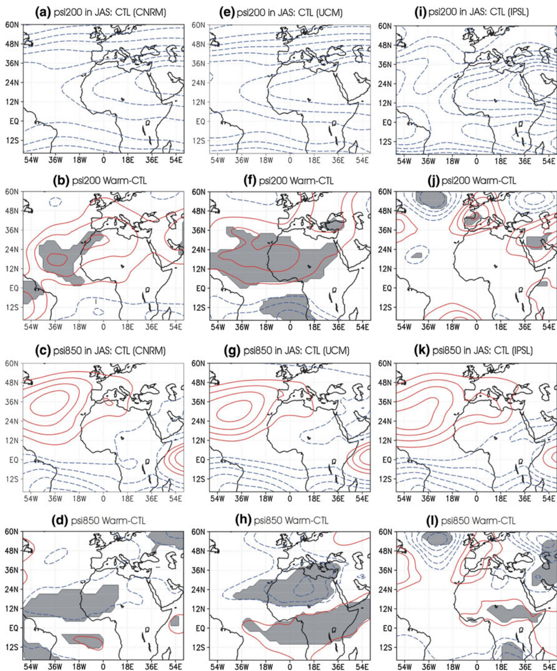
Fig. 10 July–September streamfunction composite at 200 hPa ( first and second rows ) and 850 hPa ( third and fourth rows ) from CNRM ( left ), UCM ( middle ) and IPSL ( right ). First ( ci = 1.0 \times 10^7 \text{ m}^2/\text{s} ) and Third ( ci = 3.0 \times 10^6 \text{ m}^2/\text{s} ) rows: control runs. Second
