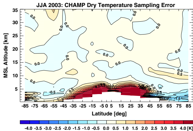
Fig. 8 Estimated dry temperature sampling error for the summer season JJA 2003. The cut-off region ( white ) corresponds to height intervals where the remaining ensemble of RO events has decreased to <10 in the respective bin
