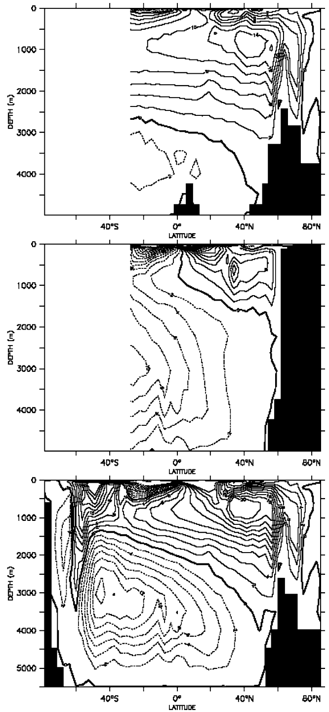
Fig. 20 Zonally averaged streamfunction for different basins for VD04 (vertical background diffusivity \kappa_v^{bg} = 0.4 \times 10^{-1} \text{ m}^2 \text{ s}^{-1} ). Atlantic basin ( upper panel ), Indo-Pacific basin ( middle panel ) and global ( lower panel )
