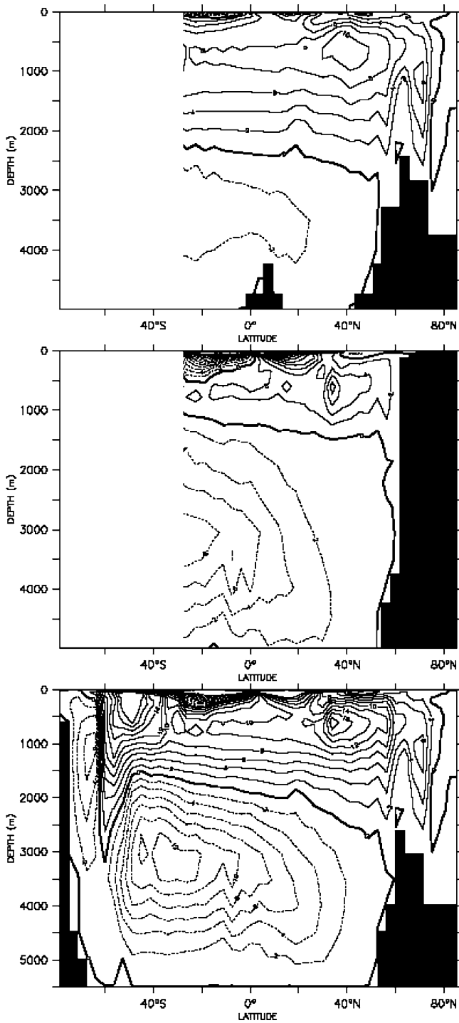
Fig. 19 Zonally averaged streamfunction for different basins for VD01 (vertical background diffusivity \kappa_v^{bg} = 0.1 \times 10^{-1} \text{ m}^2 \text{ s}^{-1} ). Atlantic basin ( upper panel ), Indo-Pacific basin ( middle panel ) and global ( lower panel )
