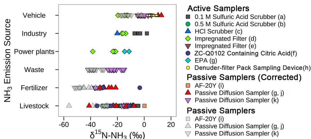
Fig. 2. The nitrogen isotopic composition of ammonia characterized at various endmembers. Recent reported isotopic signatures from traffic plumes, fertilizer and livestock (Ti et al., 2018; Kawashima, 2019; Walters et al., 2020a) were updated based on the previous summary by Walters and Hastings (2018). Note that the field sampling was conducted by different collection methods (legend) and is grouped by passive against active samplers (symbols with colors). To correct the low bias of passive data (gray symbols), 15‰ was added to the original values and is shown as corrected (symbols with colors) accordingly. Symbols with the same color and shape represent a series of observations during the same campaign. Data sources: (a) Freyer (1978); (b) Hristov et al. (2009); (c) Heaton (1987); (d) Savard et al. (2017); (e) Smirnov et al. (2012); (f) Ti et al. (2018); (g) Felix et al. (2013); (h) Walters et al. (2020b); (i) Kawashima (2019); (j) Felix et al. (2014); (k) Chang et al. (2016).
