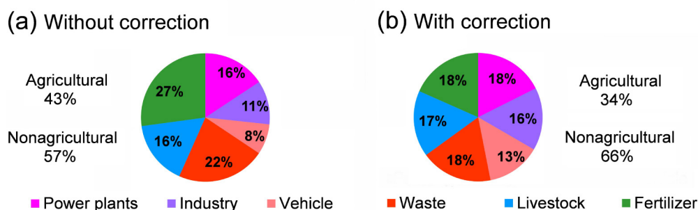
Fig. 3. Source apportionment of atmospheric ammonia in urban Beijing based on isotopic inventory (a) without and (b) with correction for the passive collection bias in characterizing nitrogen isotopic composition of ammonia, as shown in Fig. 2. The nitrogen isotopic values of -18.2\text{‰} (corrected) and -33.2\text{‰} (original) were selected as input for ambient ammonia samples. The original isotope data of -33.2\text{‰} were the annual mean values observed between March 2016 and March 2017 by Zhang et al. (2020).
