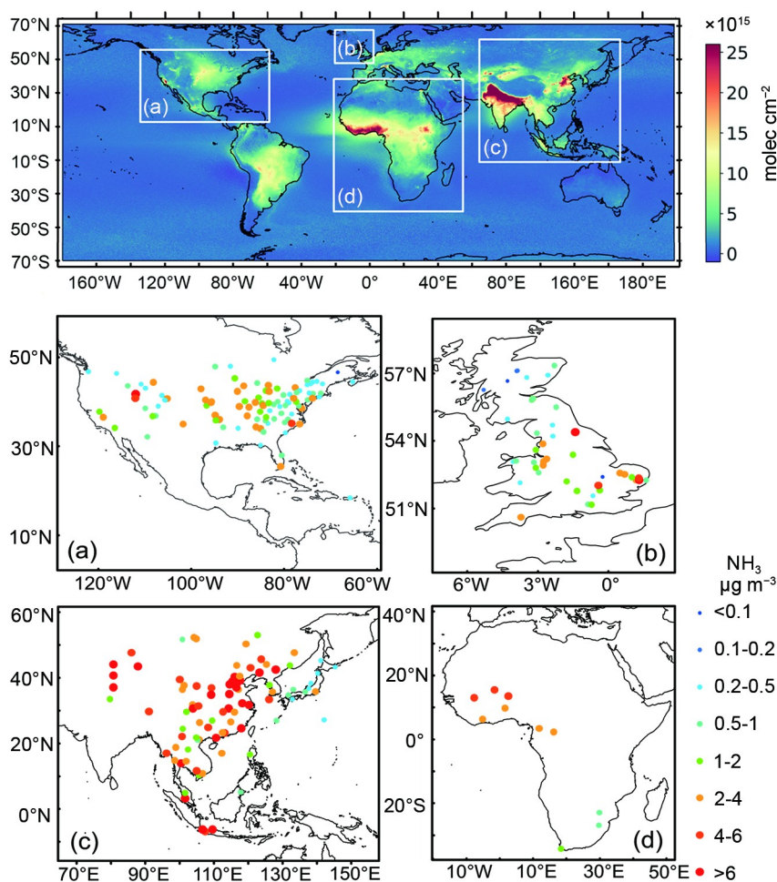
Fig. 1. Surface ammonia concentrations during 2015–16 observed by AMoN in (a) the U.S. ( http://nadp.slh.wisc.edu/AMoN/ ), (b) the UK ( https://uk-air.defra.gov.uk/ ), and (c) East Asia ( https://www.eanet.asia/ ) including China (Pan et al., 2018). (d) Long-term surface measurements of ammonia in Africa within the framework of the IDAF (IGAC-DEBITS-AFRICA) program (mean values from 1998 to 2007) (Adon et al., 2010). Global ammonia morning column measurements (2008–16) observed from space by IASI are also shown ( https://doi.pangaea.de/10.1594/PANGAEA.894736 ).
