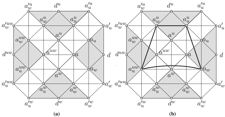
Fig. 15 A surface S studied in the proof of Lemma 7.14. If S has a corner a that is incident to two vertices of defect 0 then X contains the subcomplex illustrated in a. The cycle in b is contained in X and has no diagonal which contradicts 6-largeness
