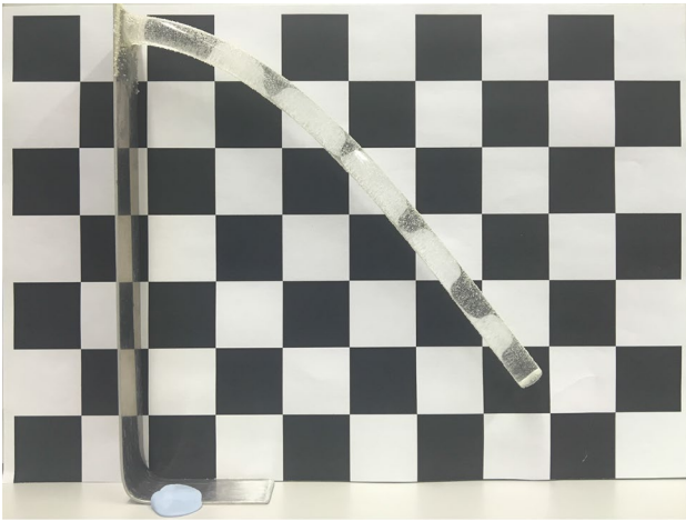
Fig. 5 Experimental setup: initially a straight PDMS cylindrical beam of 182 mm length and 8.5 mm diameter, clamped on the left side and deformed by gravity
