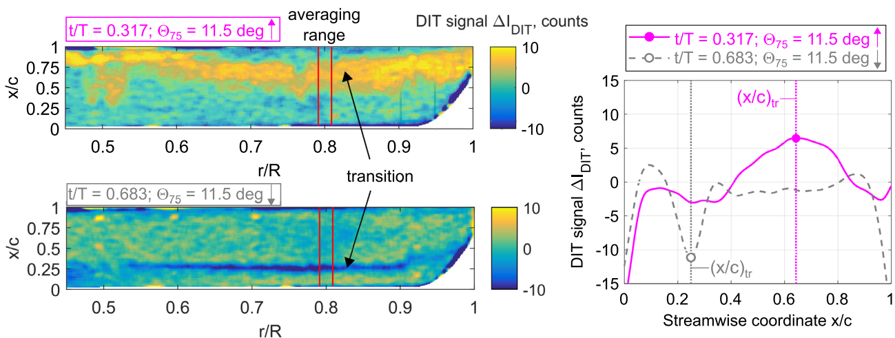
Fig. 10 DIT results for test case V (see Table 1) at an instantaneous pitch angle of \Theta_{75} = 11.5^\circ \uparrow (top) and \downarrow (bottom) with spanwise averaged DIT signals at r/R = 0.8 against streamwise coordinate (right)
