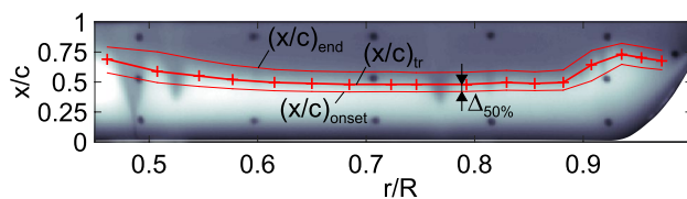
Fig. 6 Measured transition positions, transition onset and end (in red) over corresponding infrared image at \Theta_{75} = 10.0^\circ , f_{rotor} = 23.6 Hz and v_\infty = 4.9 m/s, rotation is clockwise
