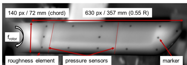
Fig. 5 Sample image acquired at f_{rotor} = 12.0 Hz, \bar{\Theta}_{75} = 10.1^\circ and \hat{\Theta} = 2.9^\circ
