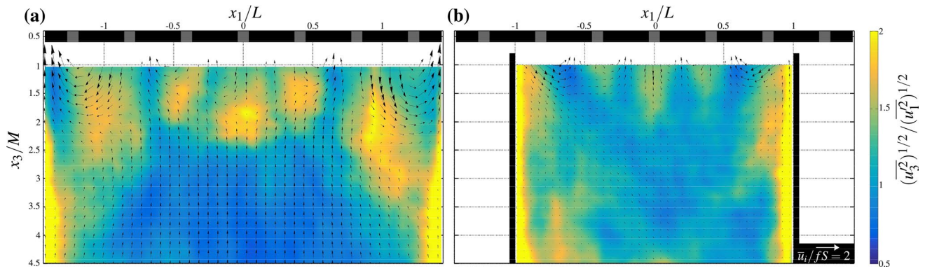
Fig. 7 Colour maps showing the degree-of-isotropy field (u_3^2)^{1/2}/(u_1^2)^{1/2} together with vector plots showing the time-averaged components of mean velocity \bar{u}_i/fS . The data shown are a Experiment A2 and b Experiment B2. In each case, Re = 4050 , f = 3.6 Hz. The same colour scale for isotropy has been used in each plot, which
