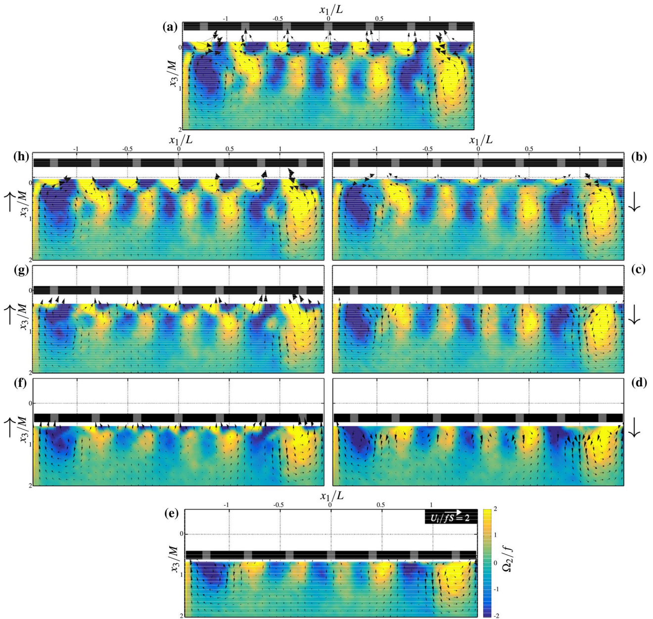
Fig. 3 Experiment A1 ( Re = 2020 , f = 1.6\text{Hz} ). Vector plots showing the ensemble-averaged mean velocity components U_1/fS and U_3/fS , together with the corresponding ensemble-averaged mean vorticity \Omega_2/f , at each of the eight grid locations x_{3,k} : a x_{3,1} = -S , b x_{3,2} = -0.71S , c x_{3,3} = 0 , d x_{3,4} = 0.71S , e x_{3,5} = S , f x_{3,6} = 0.71S , g x_{3,7} = 0 , h x_{3,8} = -0.71S . The same colour scale for vorticity has been used in each plot, which is shown in e , together with a reference
