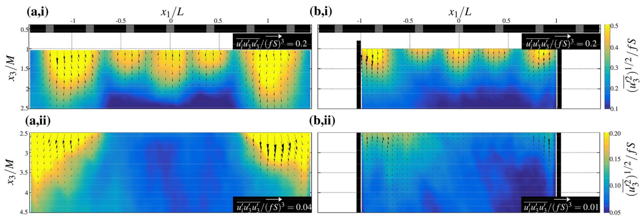
Fig. 9 Vector plots showing the time-averaged components of turbulent energy flux u'_i u'_3 u'_3 / (fS)^3 (where i = 1, 3 denote the horizontal and vertical flux, respectively), which have been superimposed on top of colour maps showing the vertical rms velocity field (u_3^2)^{1/2} / fS . The data are from a Experiment A2 and b Experiment B2 (with Re = 4050 and f = 3.6 Hz in both cases). To provide a meaningful
