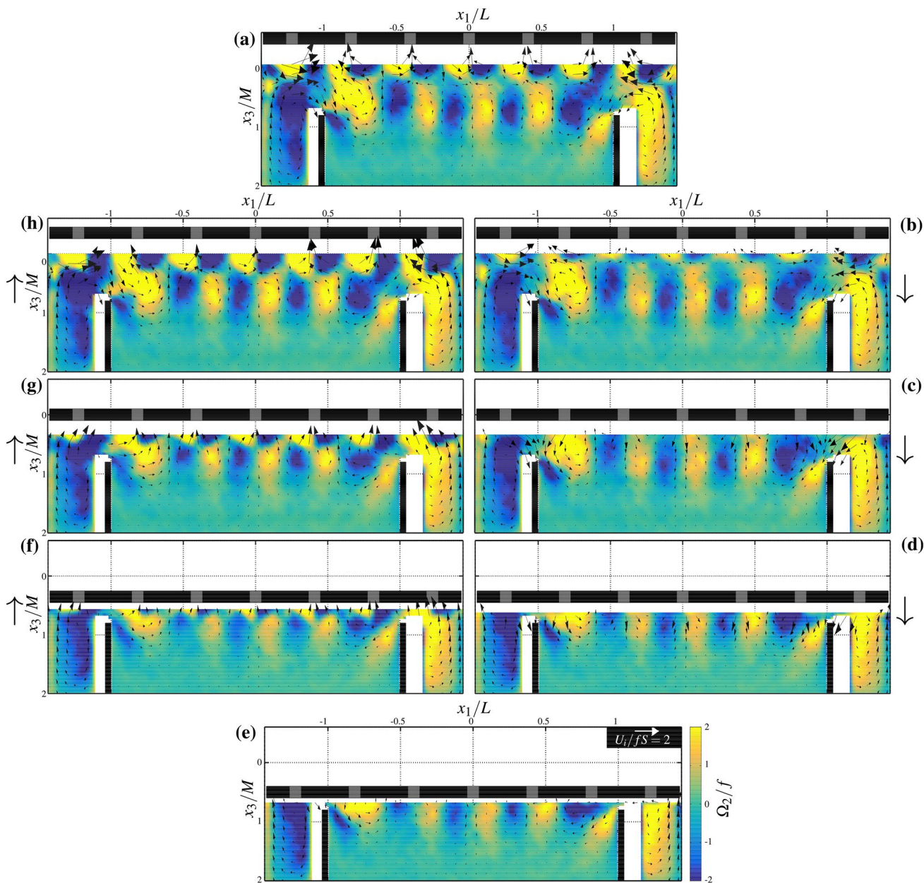
Fig. 5 Experiment B1 ( Re = 2020 , f = 1.6\text{Hz} ). Vector plots showing the ensemble-averaged mean velocity components U_1/fS and U_3/fS , together with the corresponding ensemble-averaged mean vorticity \Omega_2/f , at each of the eight grid locations x_{3,k} : a x_{3,1} = -S , b x_{3,2} = -0.71S , c x_{3,3} = 0 , d x_{3,4} = 0.71S , e x_{3,5} = S , f x_{3,6} = 0.71S , g x_{3,7} = 0 , h x_{3,8} = -0.71S . The same colour scale for vorticity has
