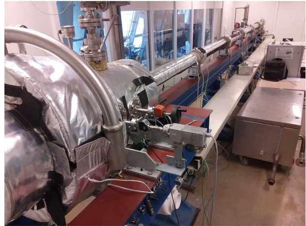
Fig. 3 Picture of the FAST set-up
