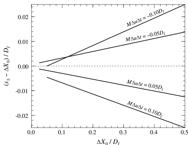
Fig. 9 The first moment of the displacement distribution for a uniaxial strain as a function of the local mean displacement \Delta X_0 , for different values of the gradient parameter a = M\Delta u \Delta t
