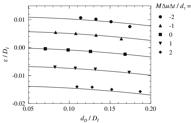
Fig. 11 The displacement bias error for uniaxial strain as a function of the correlation peak width d_D , for different values of M \Delta u \Delta t . The mean displacement \Delta X_0 is 0.25D_I . The solid lines correspond to Eq. (54); the symbols are obtained from numerical solutions of Eq. (8)
