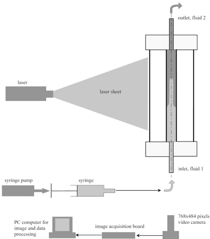
Fig. 1. Schematic diagram of the experimental setup for DPIV measurement of a more viscous fluid 2 displaced by a less viscous fluid 1 in a vertical cylindrical tube
