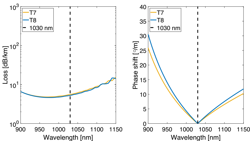
Fig. 6 Confinement loss averaged over the two orthogonally polarized fundamental modes (a) and bending-induced phase shift of fundamental modes (b) as a function of the wavelength for a perfectly linearly polarized incident beam with orientation angle \theta of 45^\circ or 135^\circ ; the bending radius was set to 0.2 m (see Fig. 1 the grey dashed line); T7 fiber: D_{core} = 40\mu\text{m} , d_{capillary}/D_{core} = 0.524 , N = 7 capillaries; T8 fiber: D_{core} = 40\mu\text{m} , d_{capillary}/D_{core} = 0.553 , N = 8 capillaries
