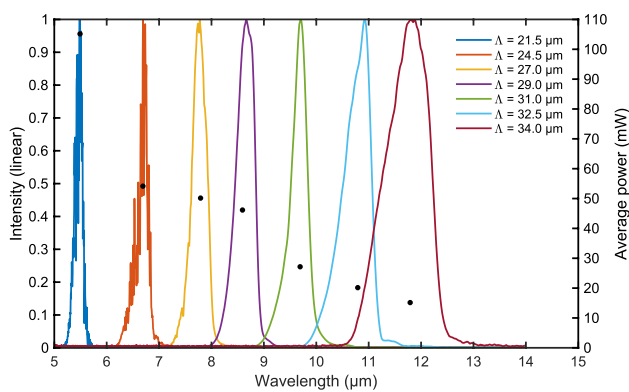
Fig. 3 Idler spectra measured at 1.2-cm -1 resolution, and average output power for seven different OPGaP grating periods
