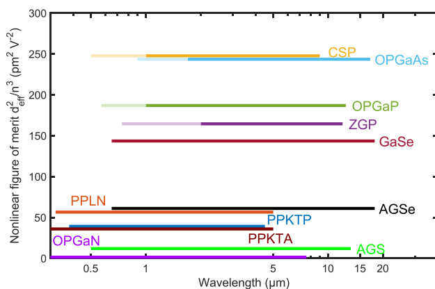
Fig. 1 Transmission range for commonly used nonlinear crystals with phasematching for mid-IR generation against their nonlinear figure of merit. This figure is adapted from [11] with additional information added on OPGaAs [12, 13], OPGaP [14, 15], ZGP [16], CSP [17, 18], PPLN [19] and PPKTP [20]. Greyed out regions show transmission which cannot be used for an OPO due to two-photon absorption or a lack of phasematching
