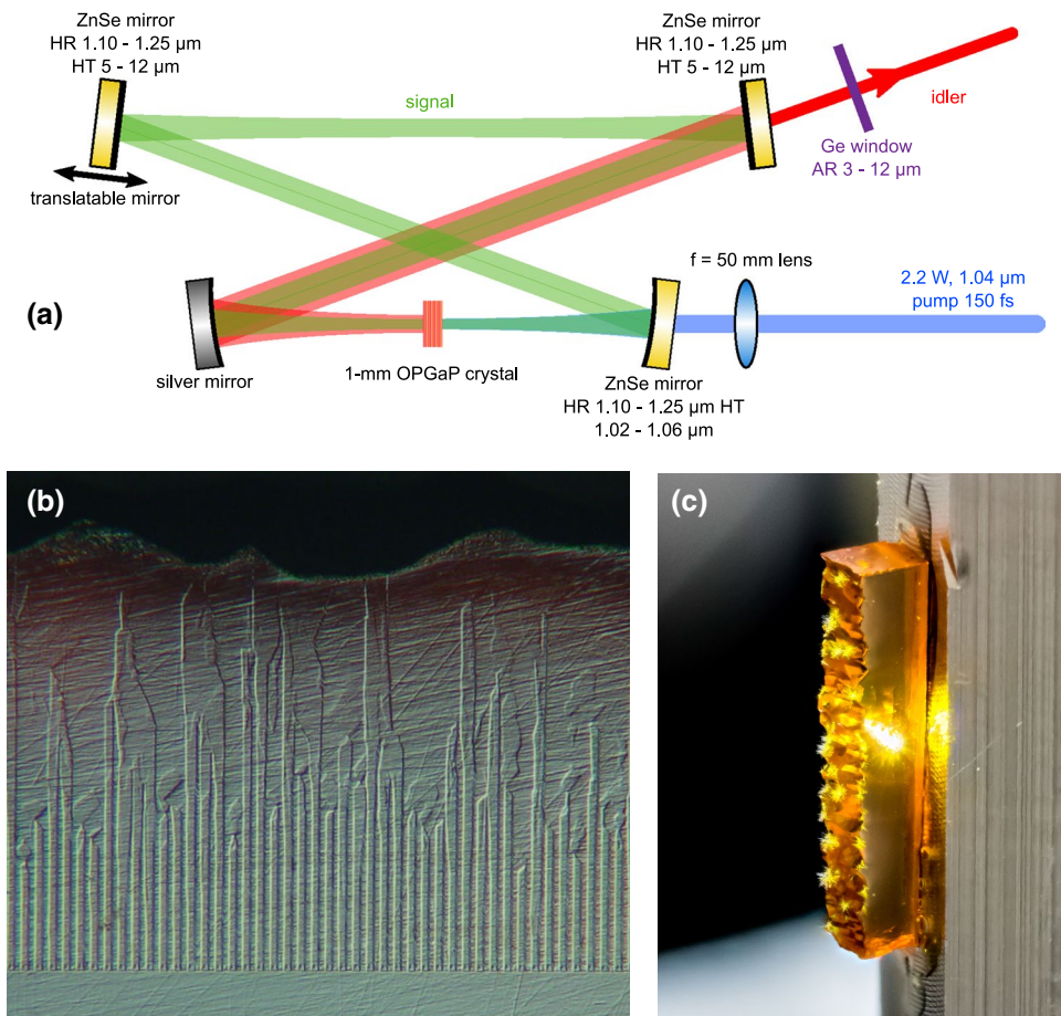
Fig. 2 a Femtosecond OPGaP OPO layout. b Microscopic cross-sectional image of 31- \mu\text{m} grating period. c Photograph of 21.5- \mu\text{m} grating period inside oscillating OPO cavity. The visible yellow light is unphasematched sum frequency generation between the signal and pump wavelengths
