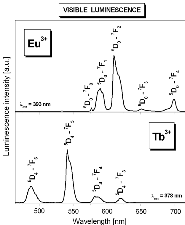
Fig. 4 Visible luminescence for \text{Eu}^{3+} and \text{Tb}^{3+} ions in lead phosphate glasses. Main red and green luminescence bands correspond to {}^5\text{D}_0-{}^7\text{F}_2 ( \text{Eu}^{3+} ) and {}^5\text{D}_4-{}^7\text{F}_5 ( \text{Tb}^{3+} ) transitions of rare earth ions
