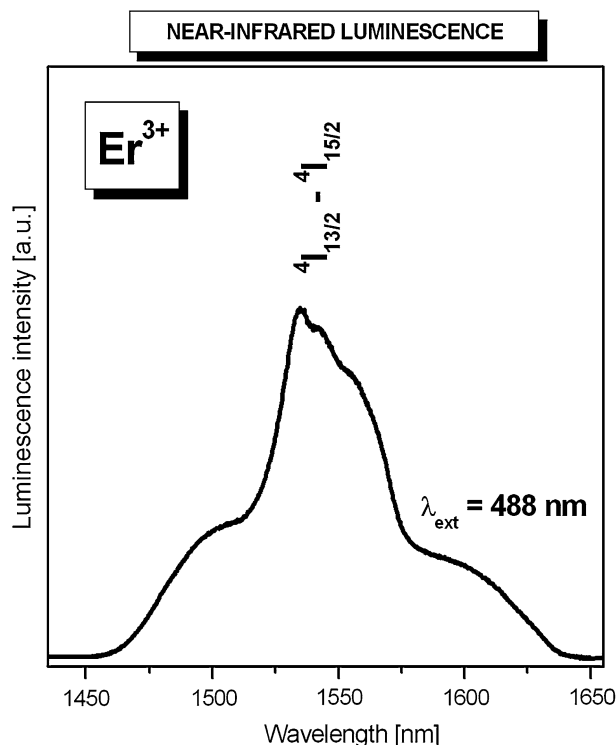
Fig. 5 Near-infrared luminescence of \text{Er}^{3+} ions in lead phosphate glass corresponding to the main {}^4\text{I}_{13/2}-{}^4\text{I}_{15/2} laser transition
