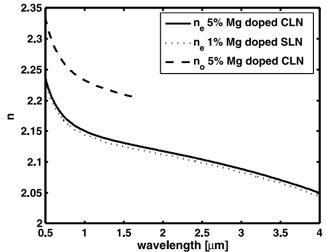
Fig. 3 Room temperature refractive index curves for 5% Mg-doped CLN ( n_e and n_o ), and for 1% Mg-doped SLN ( n_e ), according to the new Sellmeier parameters given in Table 1
