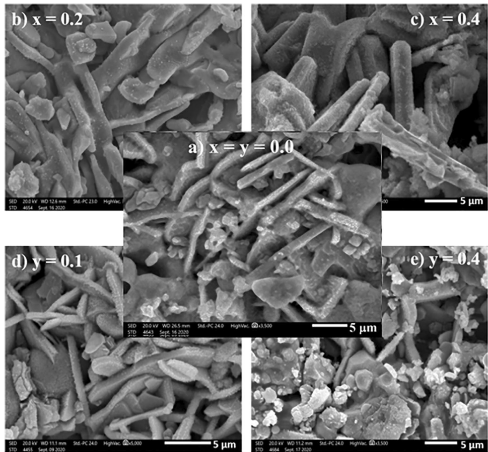
Fig. 3 SEM images of (\text{Cu}_{0.5}\text{Tl}_{0.5})\text{-1223} superconductor phase with (\text{CuF}_2)_x and (\text{TlF})_y substitutions for: a x=y=0.0 , b x=0.2 , c x=0.4 , d y=0.1 and e y=0.4
