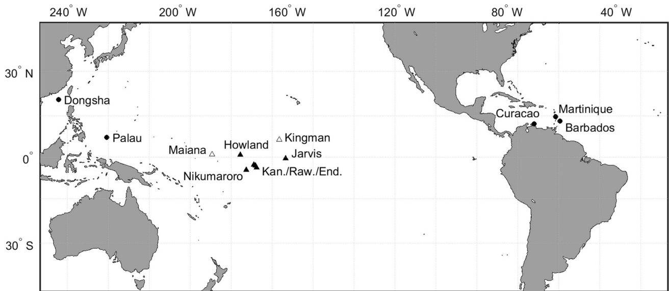
Fig. 2 Location of coral reefs included in this study. Cores collected on reefs denoted by black circles contributed to the stress band-bleaching severity calibration only. White triangles denote reefs that did not contribute to the calibration due to the absence of
