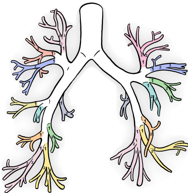
Fig. 2 The segmental branches are shown in the different colours and the numbering stands for each segmental airway generation. The segmental generation ensured all segmental bronchi started at segmental generation 1 to avoid discrepancies in the upper and lower segmental airway generations as demonstrated in Online Supplementary Material Fig. E2 (Artist: K. Rubenis)
