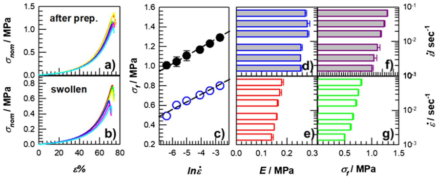
Fig. 6 a, b: Stress–strain curves depending on compression rate \dot{\epsilon} of the samples after preparation ( a ) and swollen state ( b ). c: Fracture stresses \sigma_f of the XLG-PAM-1 hydrogel after preparation (filled symbols) and swollen state (open symbols) depending on the strain rate \ln \dot{\epsilon} . d–g: Young’s moduli E and fracture stresses \sigma_f of samples at after-preparation ( d, f ) and swollen states ( e, g ) calculated at different compression rates (horizontal bars)
