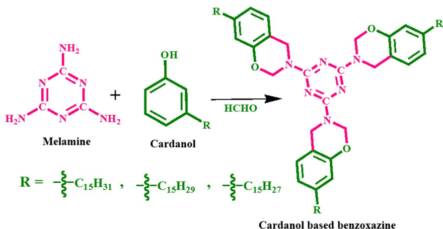
Scheme 2 Synthesis of cardanol-based benzoxazine (CBz)
