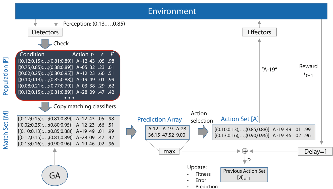
Fig. 1 Schematic illustration of the Extended Classifier System. GA Genetic Algorithm
